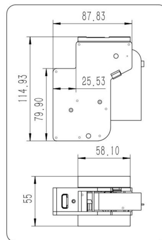
Standard Printhead
